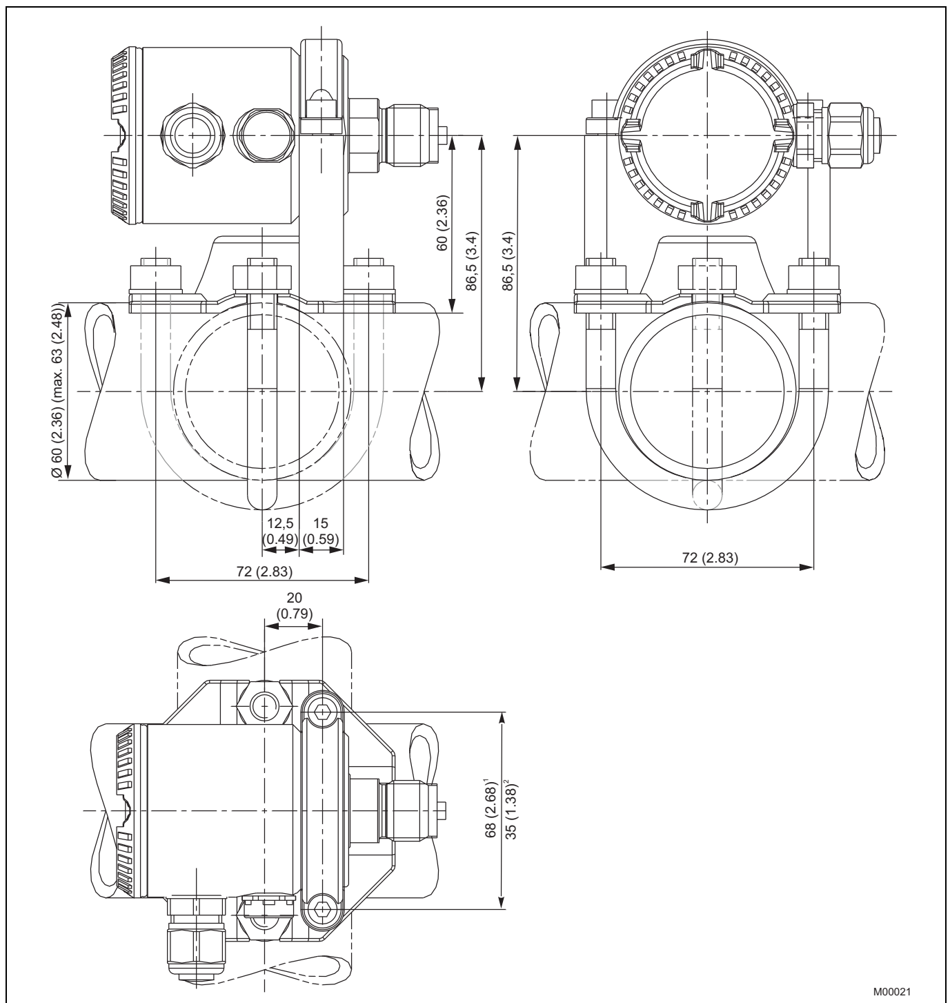
Fig. 5: Pipe/wall mounting (dimensions in mm (inches))
