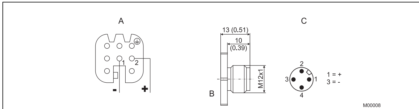
Fig. 7: Dimensions in mm (inches)
