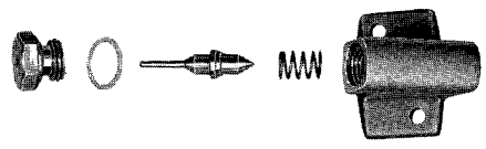
Exploded view of pilot (Note minimum of parts)
