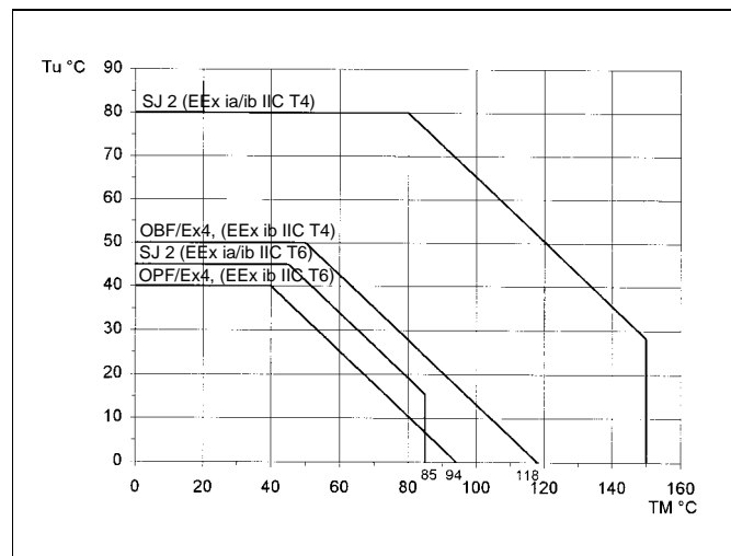
Fig. 6 10A3220/25 with Alarm Transmitter SJ 2, (EEx ia/ib IIC T4/T6, PTB No.: Ex-83/2022) and Angular Rotation Transmitter OPF/Ex4, (EEx ib IIC T4/T6, 90C.980 14X)
