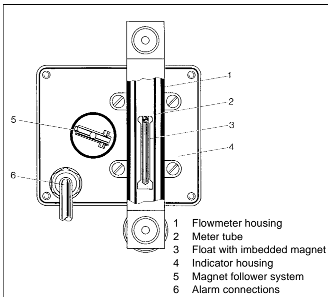
Fig. 2 Cross Section Conical Meter tube Principle
