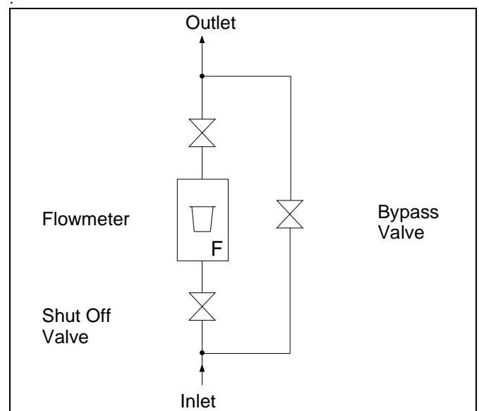
Fig. 4 Installation Example
